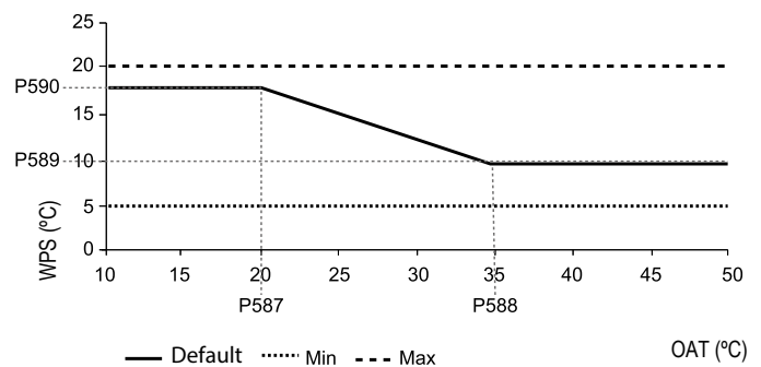
Example: Custom Cooling Climatic Curve
