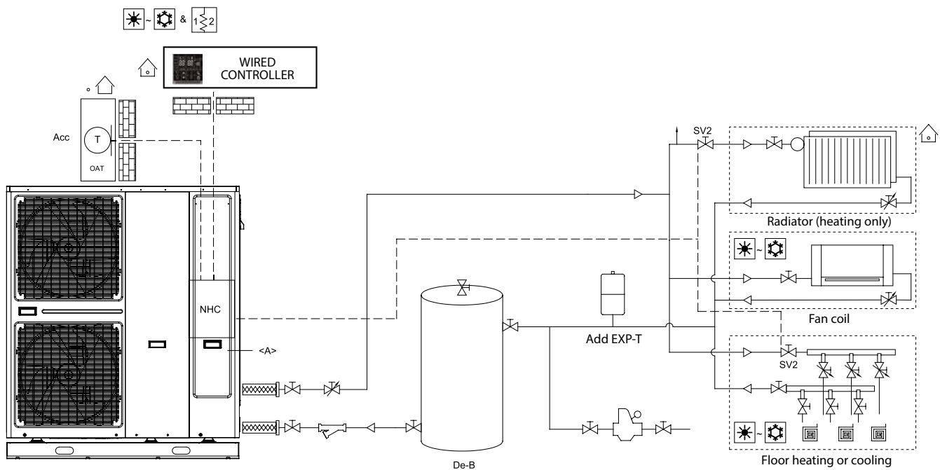
Figure: Standard installation with electric booster heater
