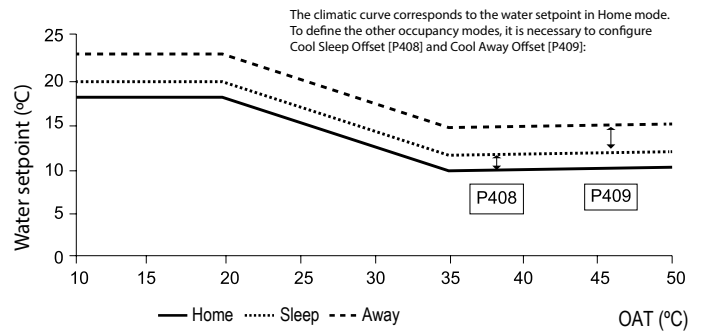
Cooling Climatic Curve in function of occupancy mode
