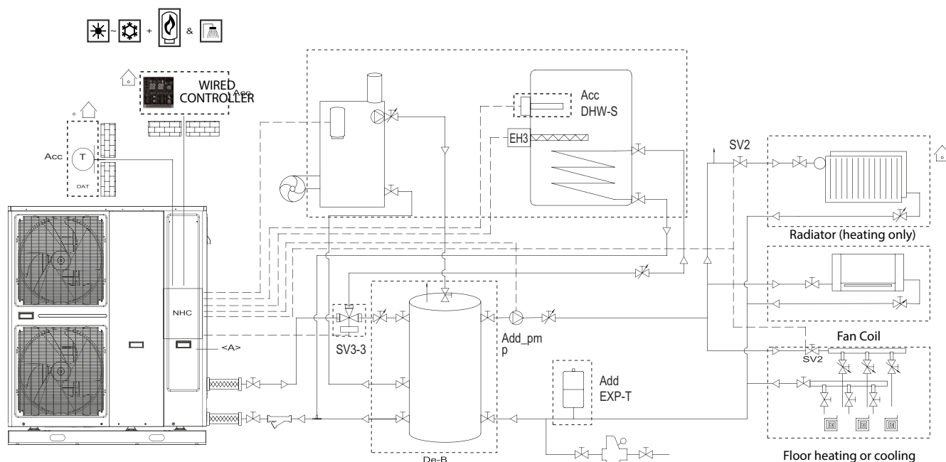
Figure: Standard installation with DHW tank and auxiliary heating source (AHS)
