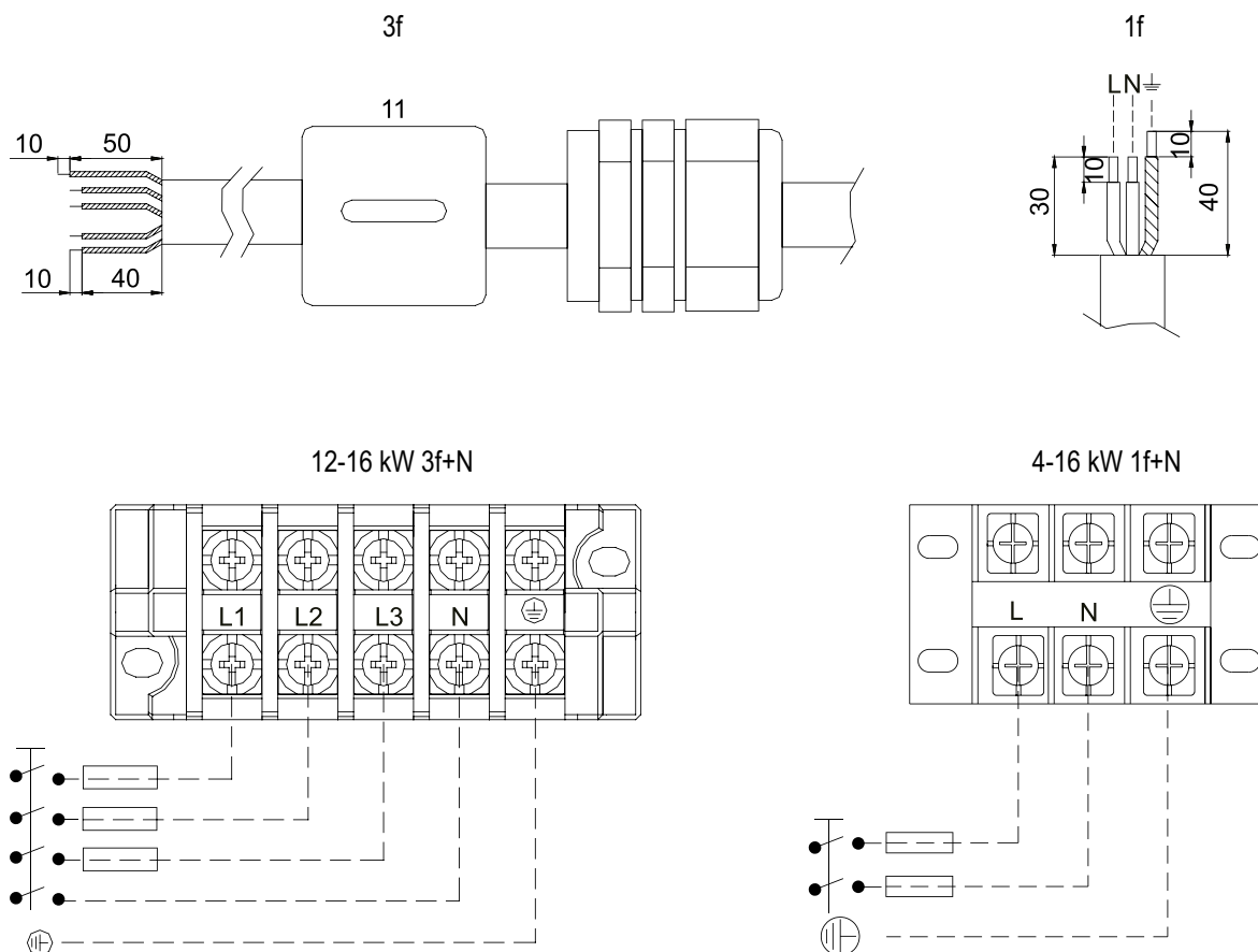
Figure 9: Power connection with Main Switch
