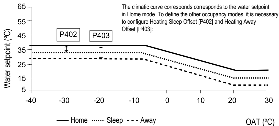
Heating Climatic Curve in function of occupancy mode
