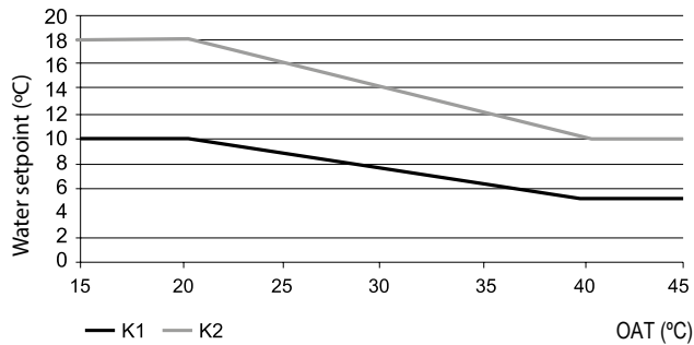
Cooling Climatic Curves
