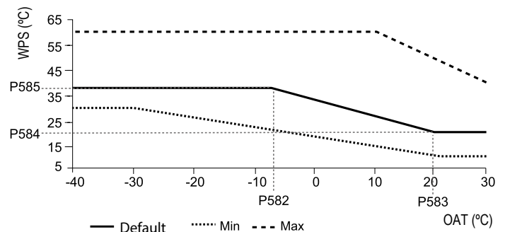
Example: Custom Heating Climatic Curve
