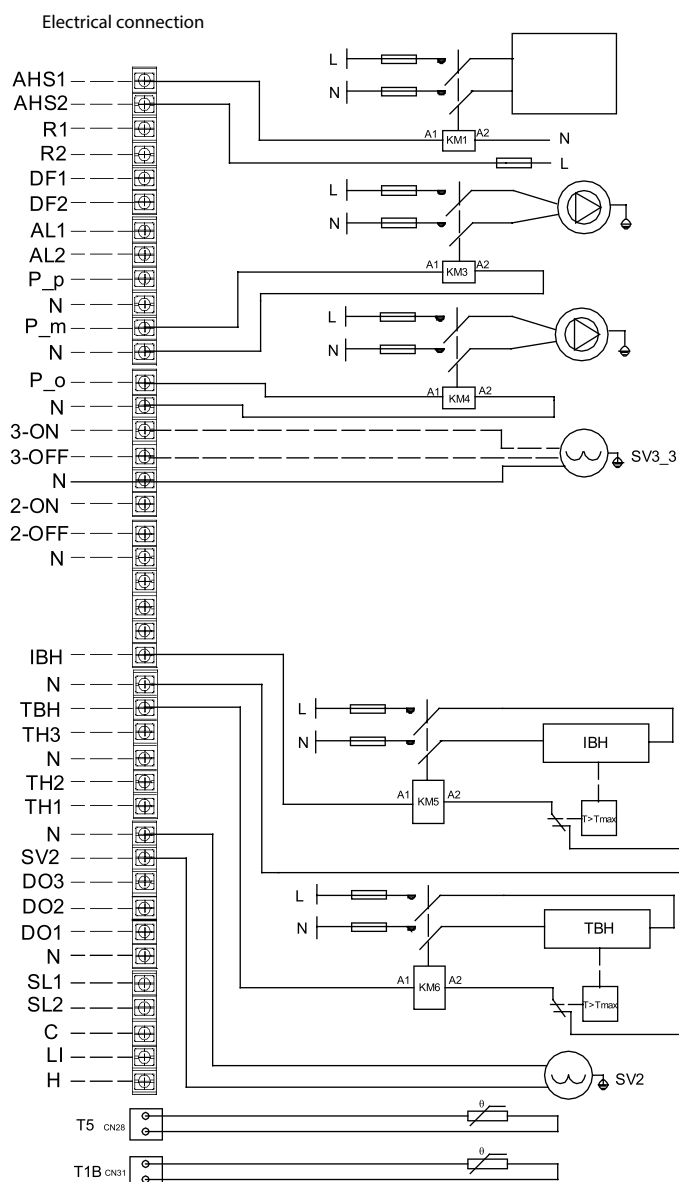
Figure: Standard installation with DHW tank and auxiliary heating source (AHS)
