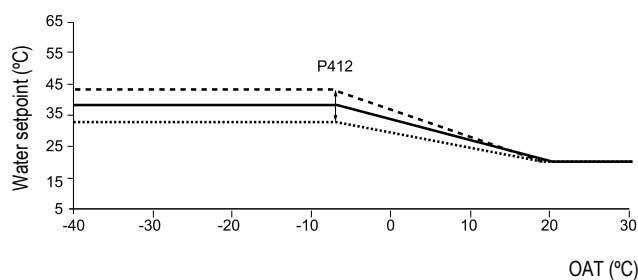
Heating Climatic Curve: Offset on head of the curve
