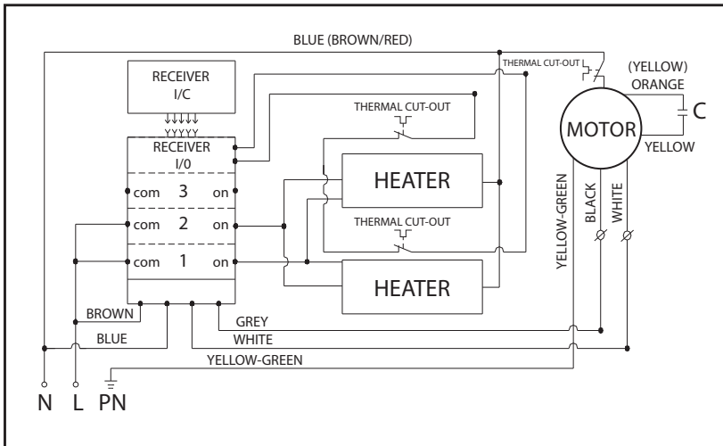
1-phase (230V~), main line: L, N
