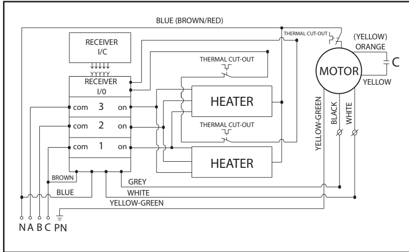
3-phase (400V~), main line: A, B, C, N
